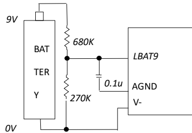
Low battery test (9V)
